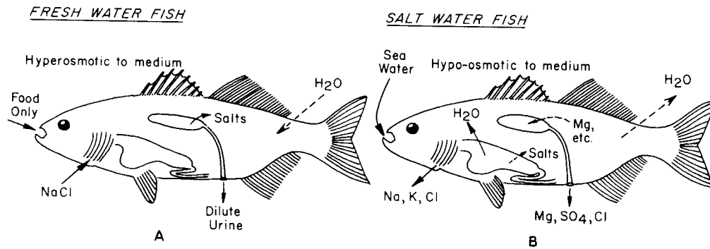
Figure 4.1.1 Schematic representation of main paths of ion and water movement in osmoregulation of freshwater bony fish, A , and marine bony fish, B . Solid arrows indicate active transport; broken arrows show passive transport.
