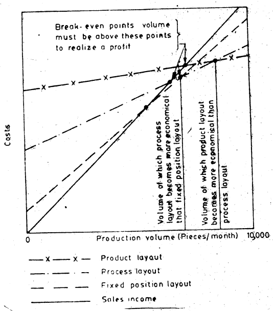
Figure III: Break-even Point Analysis of Basic Types of Layouts
