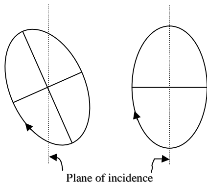
Fig.3. End on view of the reflected light from metallic mirror at (a) an angle of incidence \phi ; (b) at principal angle of incidence \phi_i
