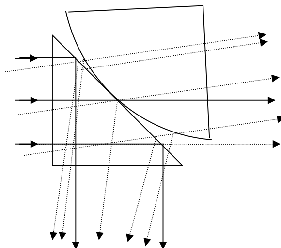
Fig 8. Hall's experiment –demonstrating that light does not undergo total reflection near the point of contact between the hypotenuse surfaces of the two prisms.
