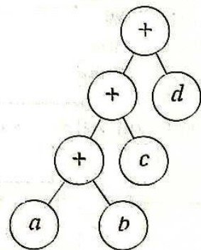
(b) ((a + b) + c) + d
